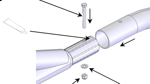
WASHER, FLAT, 5/16" I.D. HRD ZN FAS0245
