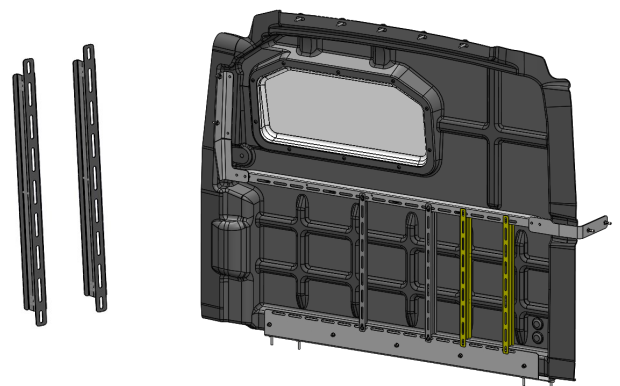
PARNHCAB (shown below in yellow) Cab side hardware mounting kit installed
