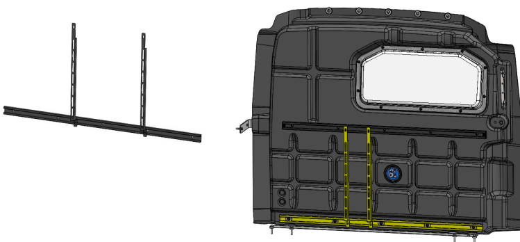
PARNHCRG (shown in yellow) Cargo side hardware mounting kit installed
