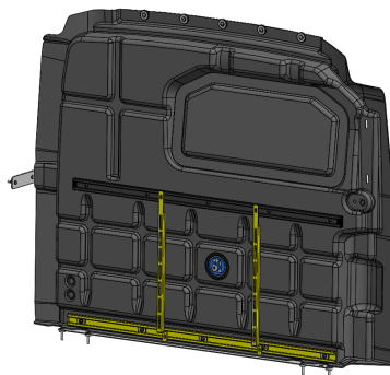
PARNHCRG (shown in yellow) Cargo side hardware mounting kit installed
