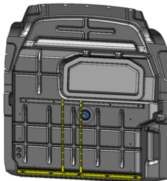
PARFTMCRG (shown in yellow) Cargo side hardware mounting kit installed
