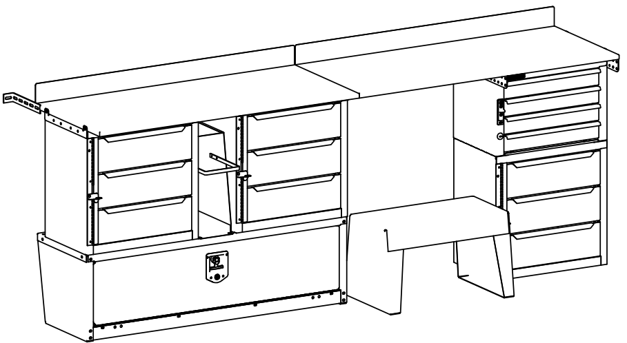
MODULAR UNIT IS SHOWN FOR STREET SIDE INSTALLATION.
