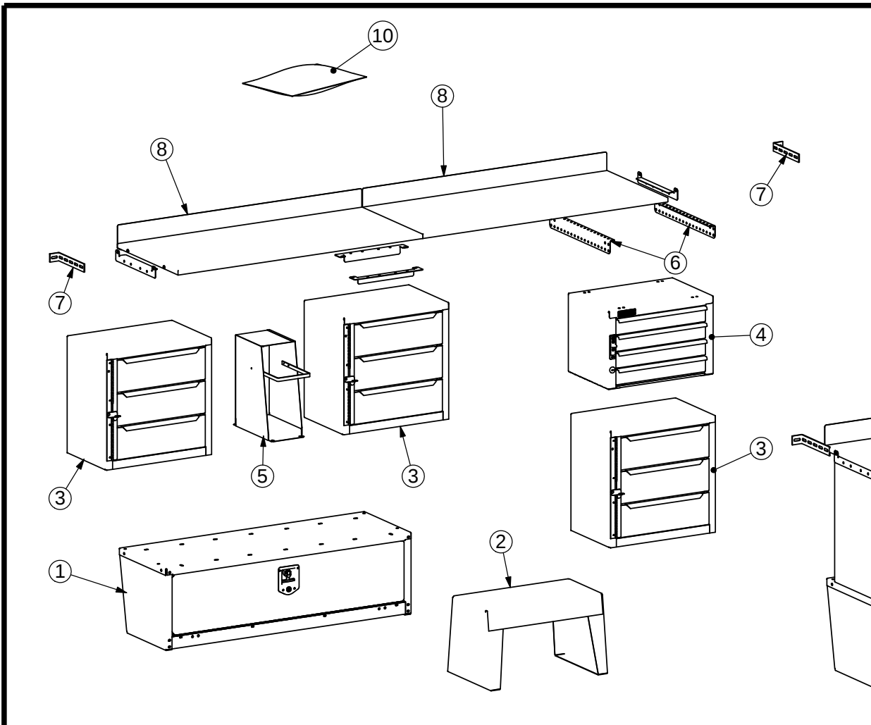
MODULAR UNIT IS SHOWN FOR STREET SIDE INSTALLATION.
