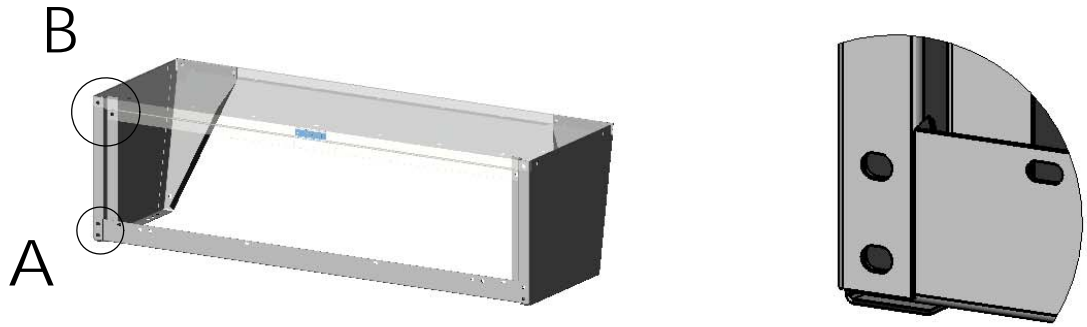
DETAIL A SCALE 1 : 2
