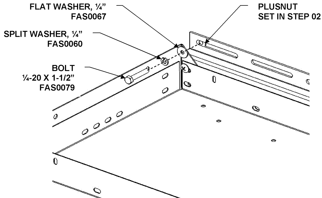
FIGURE 5. Z-RAIL FASTENING.
