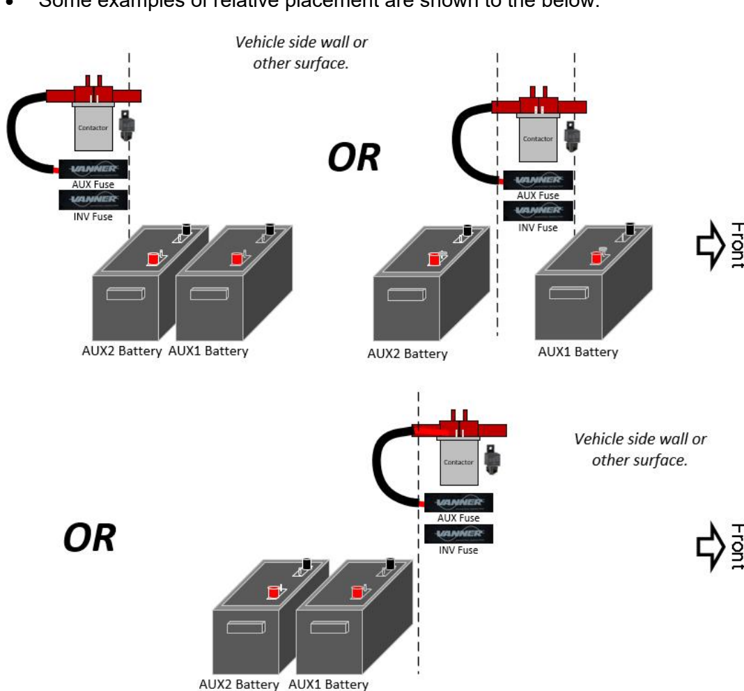
Diagram 9A-1: KIT 66007 2 AUX Battery Arrangements
