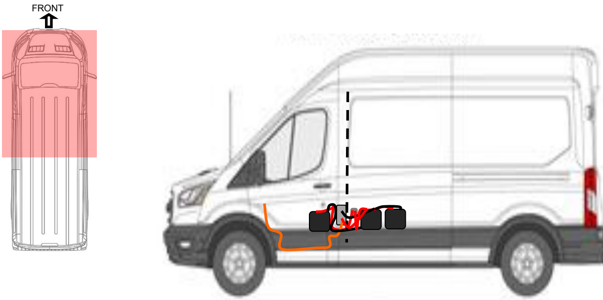
Figure 4-3: Transit Two AUX Battery Diagram
