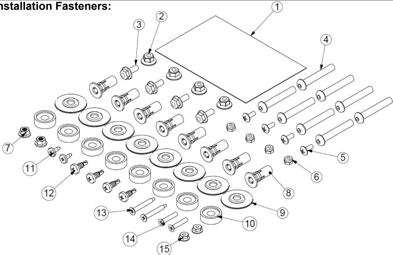
Figure 3-3: Fastener Diagram
