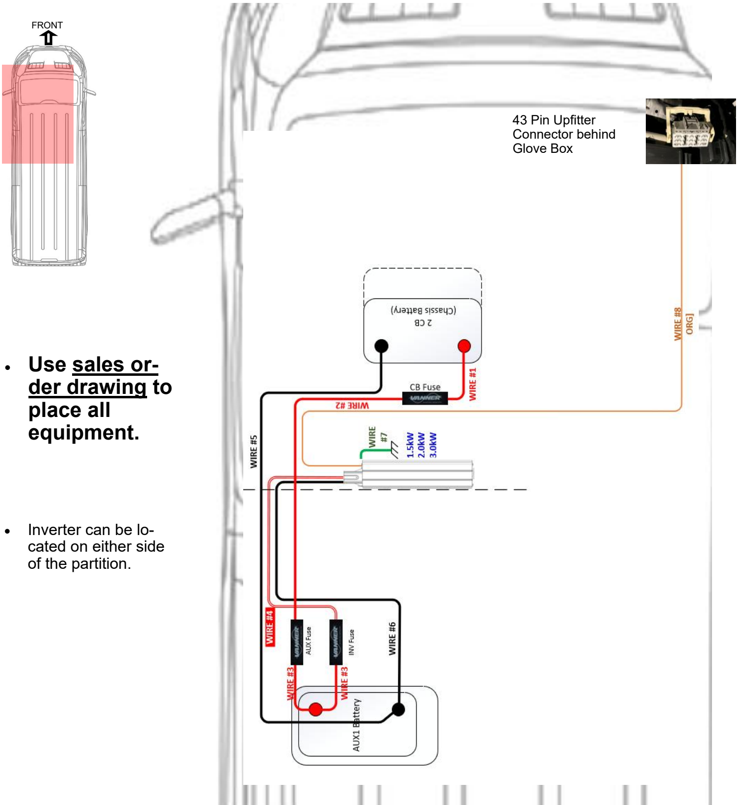
Figure 4-2: Transit NON-67C Diagram [Top]
