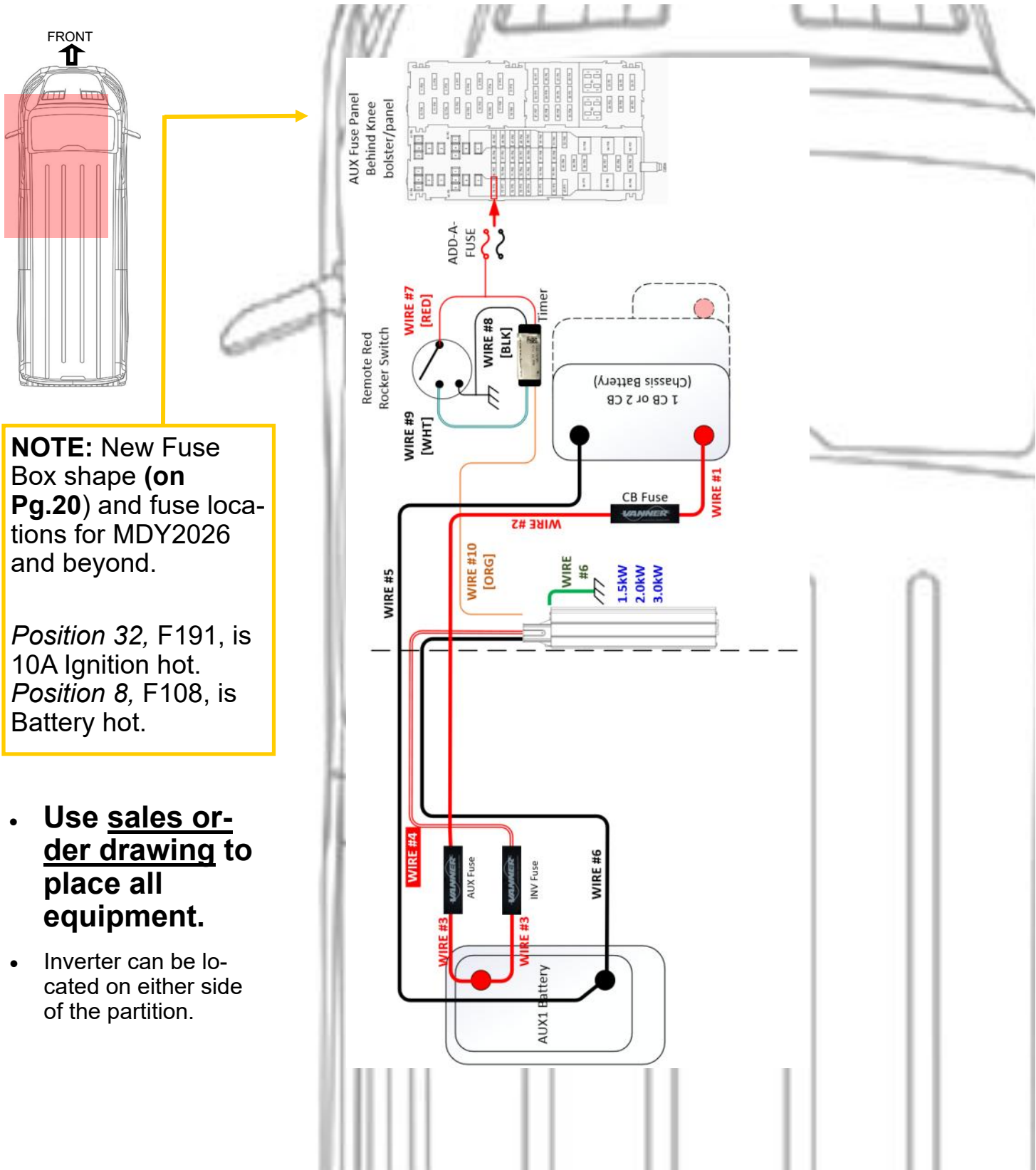
Figure 4-2: Transit NON-67C Diagram [Top]
