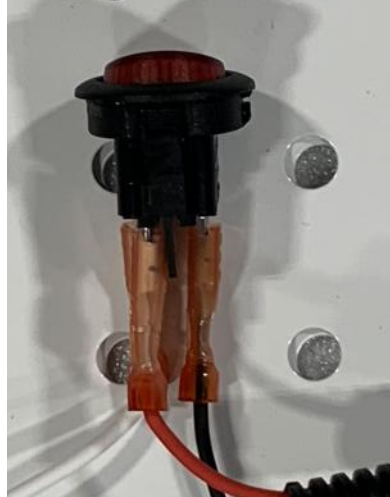
Diagram 7A-3: KIT 66008 & 66006 Remote Switch Connections
