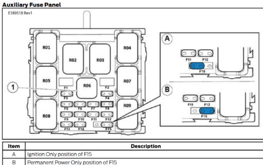
Figure 5-5: Option 67C Auxiliary Fuse Panel
