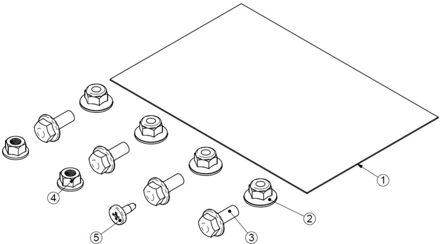
Figure 3-3: Fasteners Diagram
