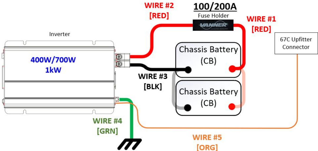
Figure 5-2: Complete Wiring Diagram [67C Option KITS 62835 & 60323]
