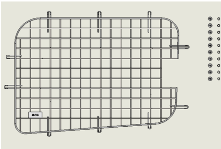
60-146 WINDOW SCREEN KIT, CURBSD (Passenger) SLIDING CARGO DOOR
