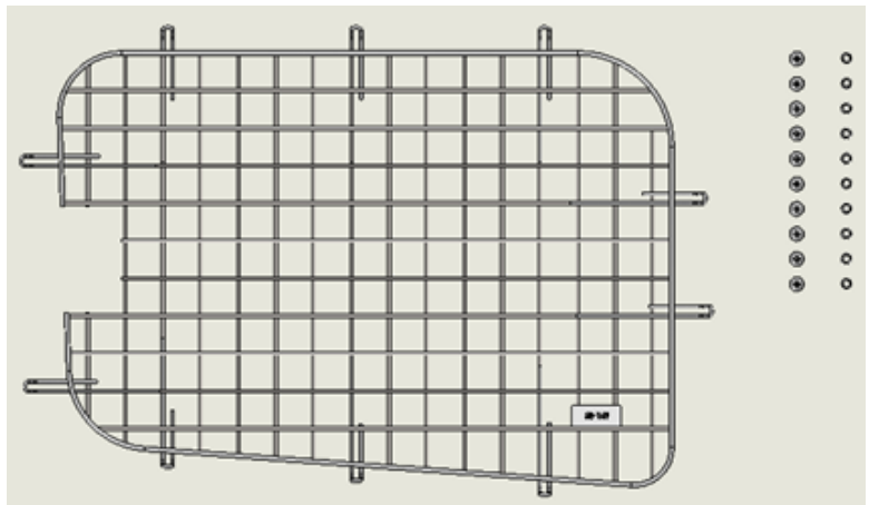
60-149 WINDOW SCREEN KIT, STREET SIDE (Driver) SLIDING CARGO DOOR
